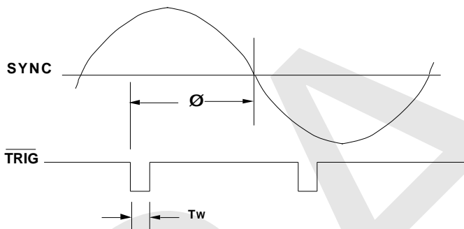
FIGURE 3. LS7634 TRIG, ∅ vs TOUCH (SENS OR EXT)
